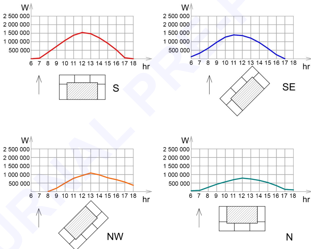
Figure 2. The amount of direct solar radiation hitting the horizontal surface of the yard, depending on the orientation with respect to the cardinal points, considering the shading Source: own work.
